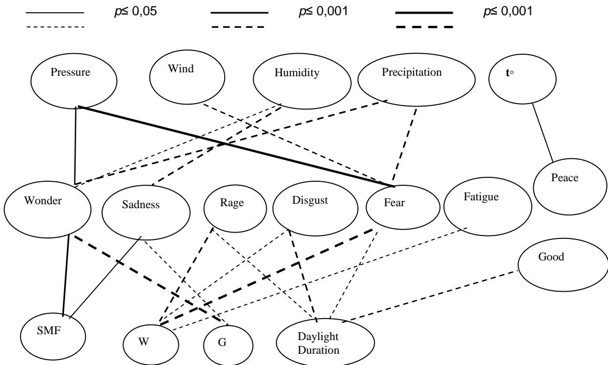
Pic.1. Correlations constellation for averaged values for 12 names in 12 days in the period of Feb 1- Apr 5, 2013.
