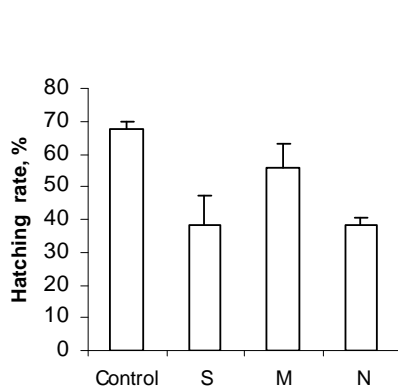
Fig. 1. Effects of constant magnetic field on Artemia hatching (S-, N-polarization, M – between them)
