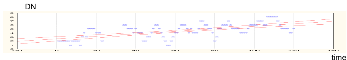
Fig. 2. The dependence of the DN (explained in the text) versus time (days) to 4.12.12 on 02.04.13.
