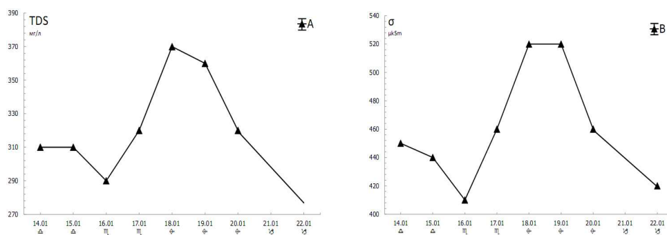
Fig. 1 Changes in the parameters \sigma and TDS of the "Ordana" water.
