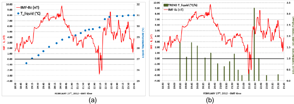
Fig. 2 The striking jump of the liquid temperature (a) and heating rate (b) in the 10-15 min following two close strong inversions of B_z having on average very large positive values, on February 27 th , 2012
