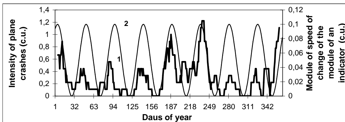
Fig. 1. Comparison of distribution of intensity of plane crashes (a curve 1) and variations of the module of speed of change of the module of an indicator (SRE or nutation deviation, a curve 2) within a year
