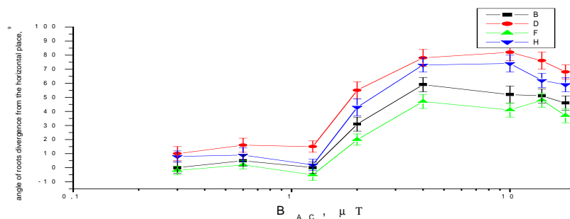
Fig. Dependence of angle of root divergence from the horizontal place at the frequency of alternative component of magnetic field f = 6.85 \text{ Hz} on the amplitude of the alternative component of magnetic field.
