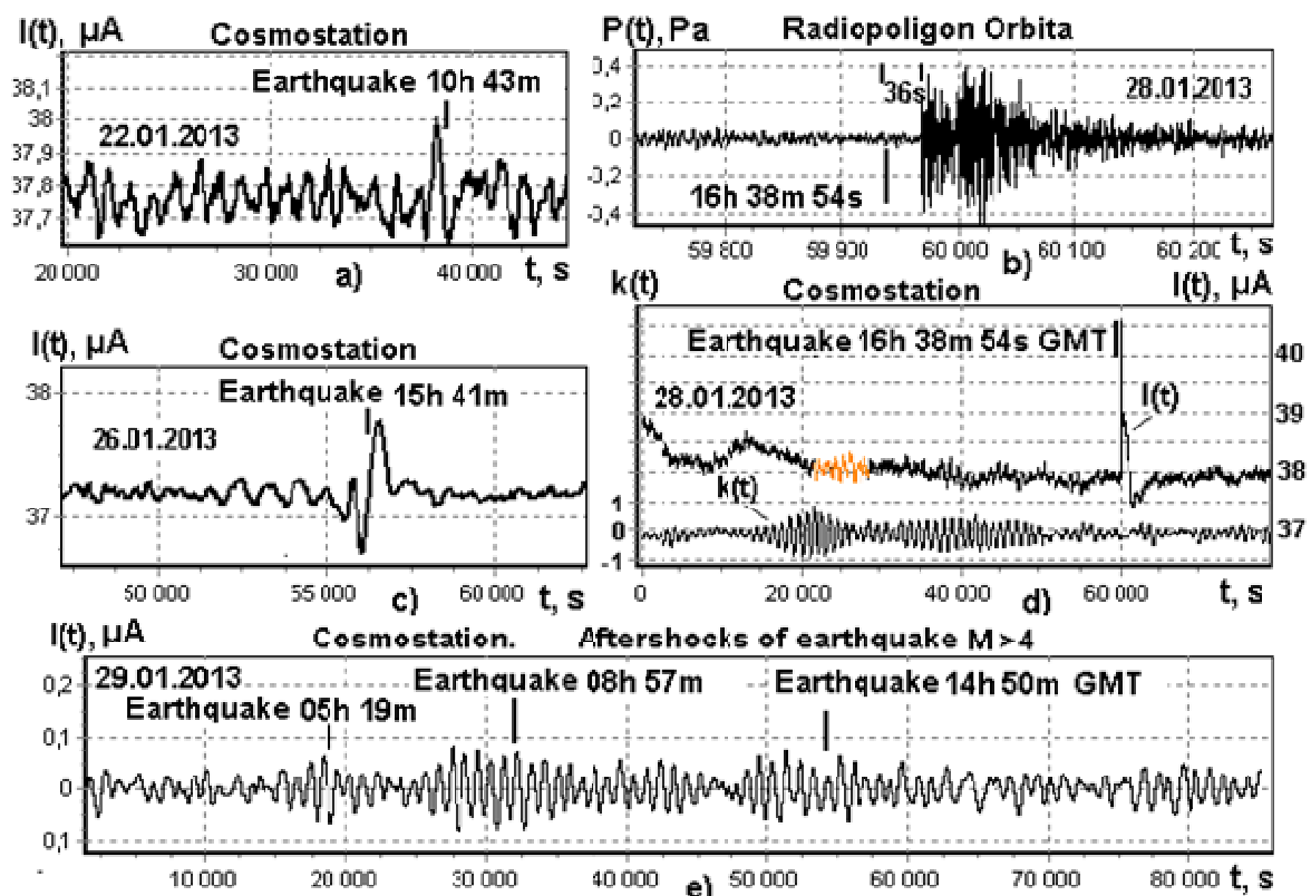
Figure 1 - Current variation I(t) in a EWC on 22.01.2013 - (a); Infrasonic signal from the earthquake M = 6,1 - (b); Current variation in a EWC on 26.01.2013 - (c); Current variation in a EWC and result of auto-correlation analysis k(t) on the eve of and during earthquake on 28.01.2013 - (d) and aftershocks on 29.01.2013 - (e). Axis X - time from the beginning of day on GMT time in seconds.
