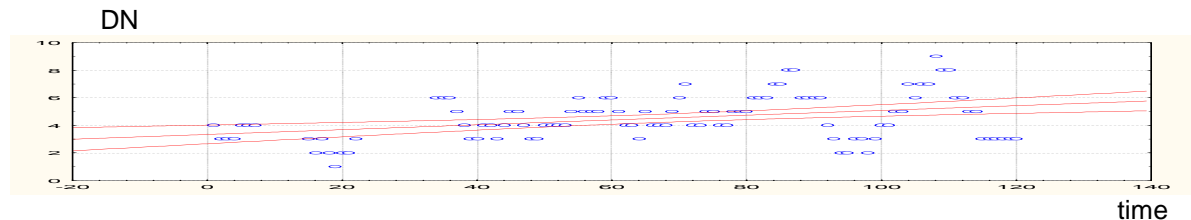
Fig. 1. The dependence of the DN (explained in the text) versus time (days) to 4.12.11 on 01.04.12.
