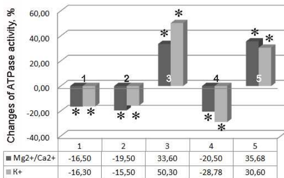
Fig. Change of \text{Mg}^{2+}/\text{Ca}^{2+} - and \text{K}^{+} -ATPase activity (%) over time under the influence of ELF EMF ( n = 50 ). * - Significant differences relative to control values, p < 0.05 .
